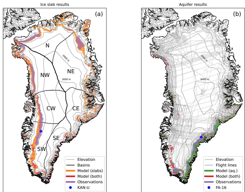
Figure 1. Locations with modeled and OIB observed (a) ice slabs for 2010–2018 (Jullien et al., 2023), and (b) aquifers during 2010–2014 (Miège et al., 2016). Full black lines in (a) represent Mouginit et al. (2019) ice sheet basins. Gray lines are OIB 2010–2018 flightlines. Blue dots represent locations of the arrows in Figure 4. Dashed gray lines indicate elevation contours at 500 m intervals.
