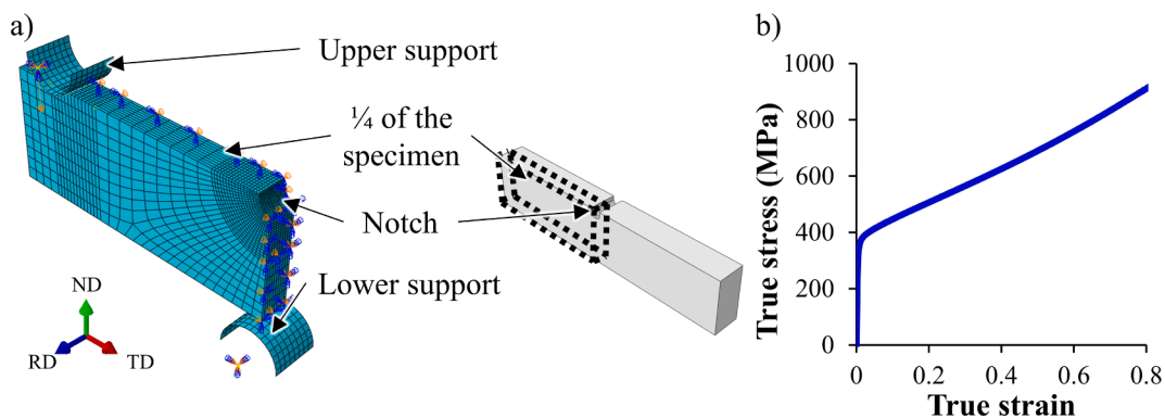
Fig. 3. A) assembly used to simulate the 3-point bending test on a quarter part of the miniaturised specimen, boundary conditions and mesh included, and b) true stress-true strain curve of the cu-30%zn implemented in the simulation.
