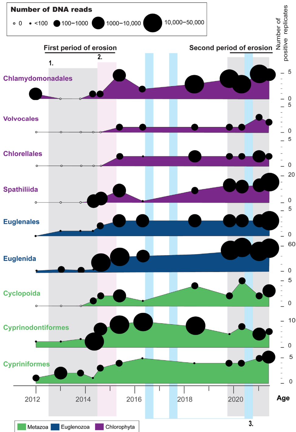
Fig. 7. Responses of aquatic communities to anthropogenic and climatic stressors. Evolution of the relative abundance of orders from the Metazoa, Euglenozoa, and Chlorophyta taxonomic groups. The size of the circle is proportional to the number of reads. The gray stripes (1) correspond to the deforestation periods, the pink stripe (2) to the main episode landscape fragmentation, and the blue stripes (3) to the main water crisis periods.
