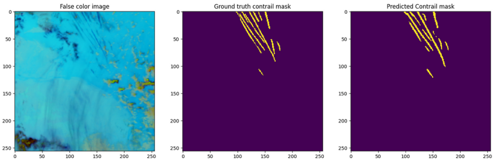
Figure 1. Example of contrail prediction by the deep segmentation model on a GOES-16 satellite image: the false color satellite image (left), the labeled image (middle) and the deep leaning prediction (right).
