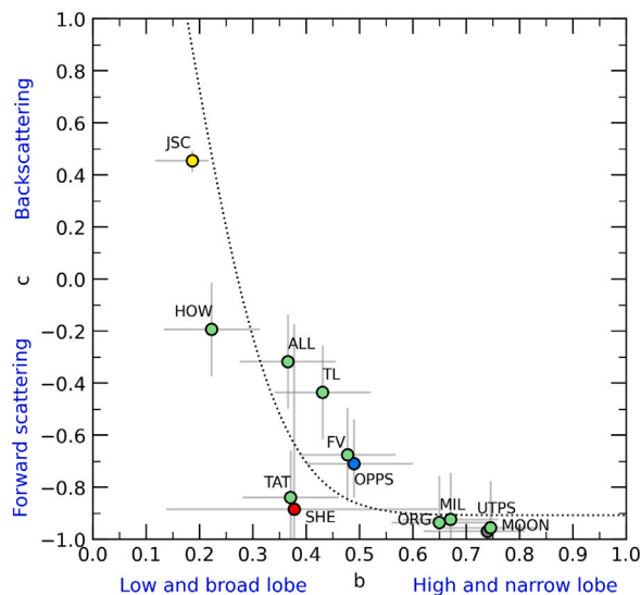
Fig. 15. Asymmetry parameter c as a function of the shape parameter b . The dotted line represents the hockey stick relation (Hapke, 2012).
