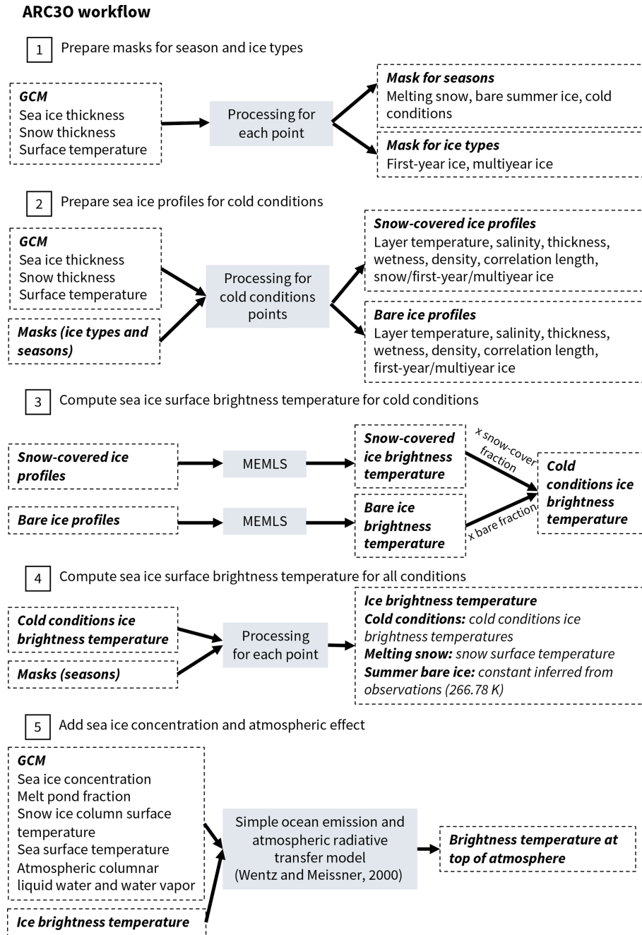
Figure 1. Workflow of the Arctic Ocean Observation Operator ARC30.
