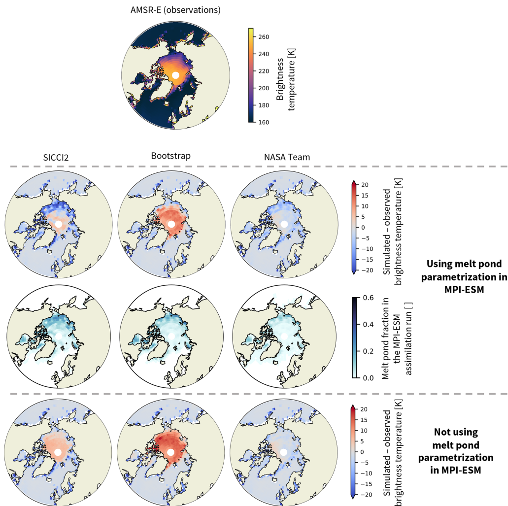
Figure 9. Experiment to compare brightness temperatures in summer (July–August–September) simulated based on assimilation runs assimilated with different sea ice concentration products (SICC12, Bootstrap, NASA Team) to brightness temperatures measured by AMSR-E. Observations by AMSR-E are shown in the first row. The difference between simulated and observed brightness temperatures if melt ponds are taken into account (second row) and if they are set to zero (fourth row) is shown. In the third row, the melt pond fraction simulated by MPI-ESM is shown.
