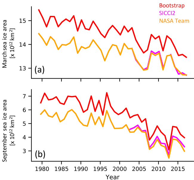
Figure 7. March (a) and September (b) sea ice area for the three observational datasets assimilated in the three assimilation runs used.
