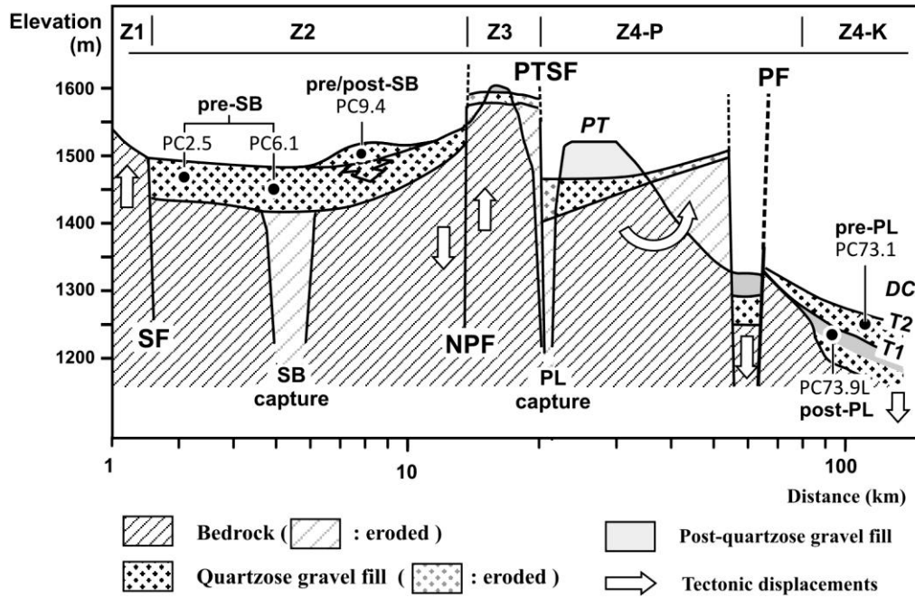
Figure 10. Sketch longitudinal profile of the Cahabón River valley, showing the spatial relationship between the selected locations for sediment dating, the capture sites and the faults. Zones Z1 to Z4 correspond to the lithology groups used for the sediment provenance analysis (see the Sediment Provenance section in the methods section). SF: Salamá Fault, NPF: Niño Perdido Fault, PTSF: Purulhá trough South Fault, PF: Polochic Fault, DC: Depression of Cobán.
