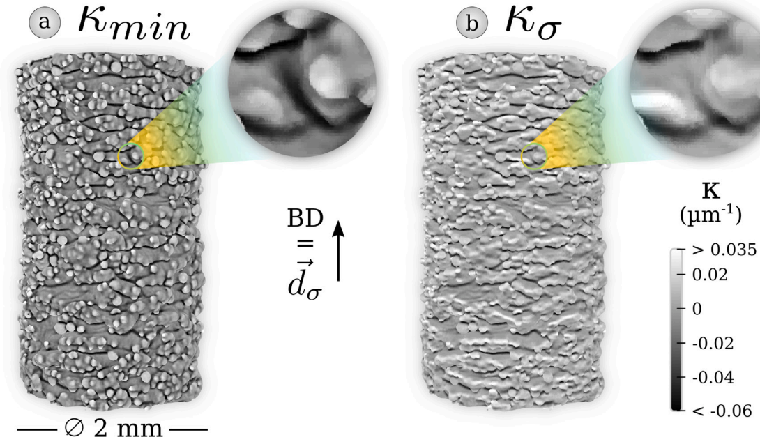
Fig. 10. (a) \kappa_{min} and (b) \kappa_{\sigma} measurements on an as-built cylindrical sample fabricated by E-PBF. Computations were made from an XCT scan with a voxel size of 5 \mu\text{m} , using r_{curv} = 30 \mu\text{m} = 6 \text{voxels} and \lambda_S = 0.025 \text{mm} = 5 \text{voxels} . The magnifying windows provide an enlarged view on a notch parallel to \vec{d}_{\sigma} . It shows that \kappa_{\sigma} manages to ignore it, whereas notches perpendicular to the loading direction are kept.
