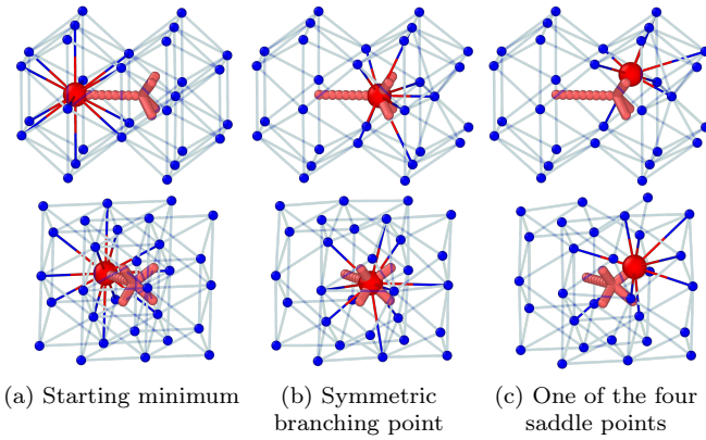
FIG. 10. Diffusion of a substitutional Cu atom (red ball) in cubic Aluminium (blue balls) by a pushing mechanism. The small pink balls represent the positions of the Cu atom in the valleys linking the starting minimum to the 4 saddle points. (10a): The starting Cu position is a substitutional site. (10c): Only one saddle point is represented. At the branching point (Fig. 10b), which is not a saddle point, the lowest eigenvalue is negative and four times degenerate. The top and bottom panels represent the same structure from two different points of view.
