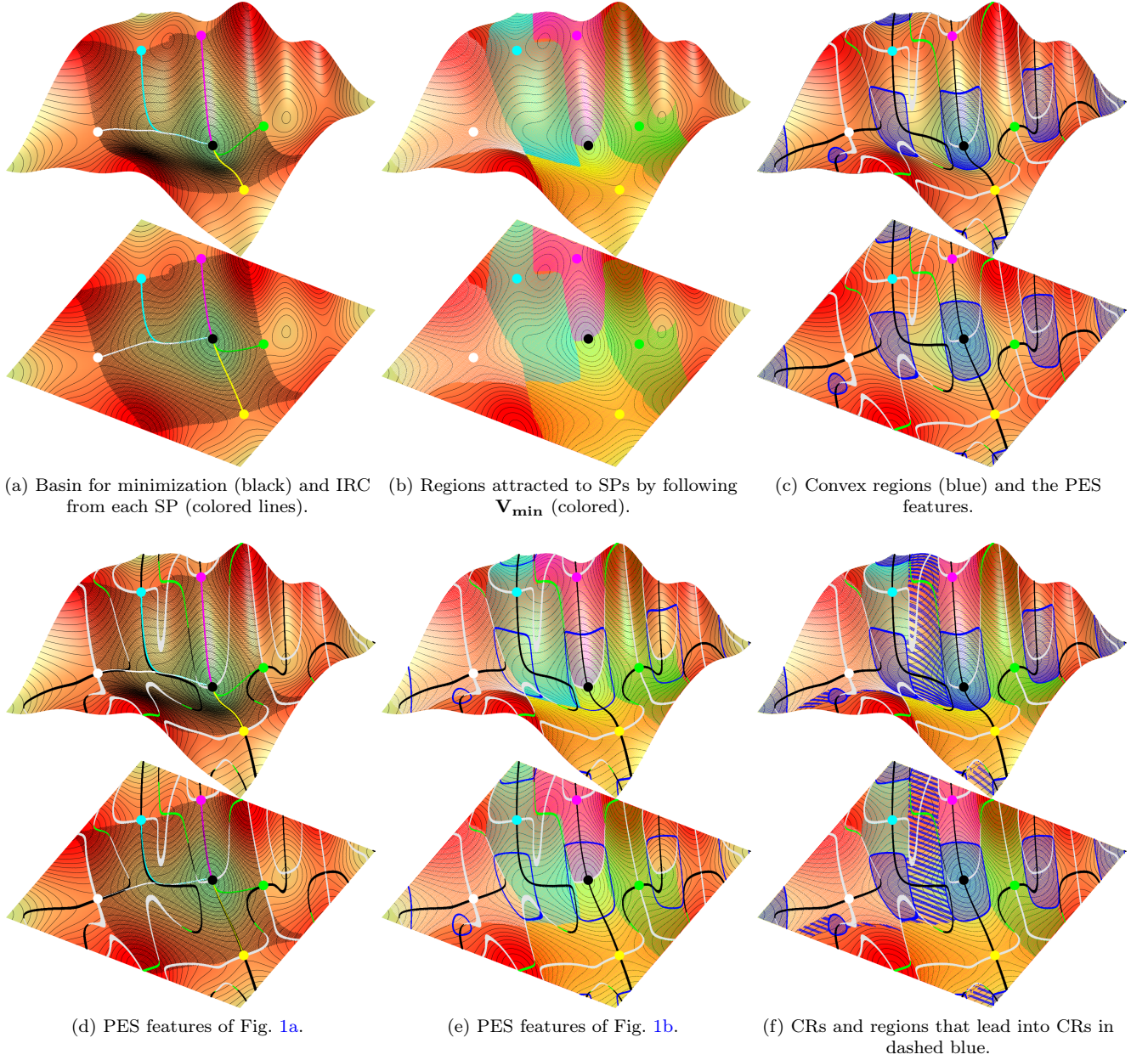
FIG. 1. Analysis of a 2D example PES where typical features can be found. The big points represent stable structures where \mathbf{F} = 0 : minimum (black) and saddle points (colored). The regions of the PES colored in a certain way represent the set of points having the same characteristics: (1a, 1d): (black) basin for minimization, (colored lines) IRC. (1b, 1e, 1f): regions attracted to SPs of the same color. (1c, 1d, 1e, 1f): PES features, valleys (black), ridges (green), perpendicular hyperplanes (gray) and inflection hyperplanes (blue), as described in Sect. II. (1f): (dashed blue) the regions that lead to a CR by following \mathbf{V}_{\min} . The analytical value of the PES is E(x, y) = \frac{1}{2} \cos(\frac{xy}{5}) \cos(\frac{3x}{5}) \cos(\frac{y}{2}) + \cos(x) \cos(\frac{3y}{2}) + \exp(-\frac{(x-17)^2 + (y-17)^2}{125}) for x \in [13; 18] and y \in [14.7; 18.6] .
