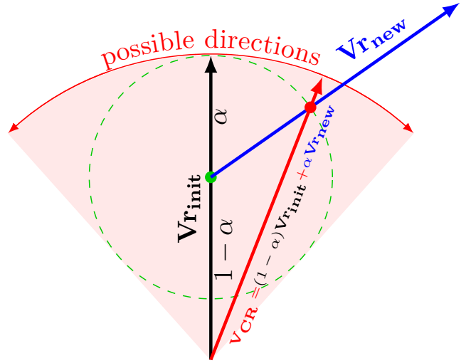
FIG. 4. Black vector \mathbf{V}_{\text{init}} : starting random vector pointing away from the initial minimum. Blue vector \mathbf{V}_{\text{new}} : new random vector reinitialized each time a CR is detected; it can point anywhere. Red vector: \mathbf{V}_{\text{CR}} = (1 - \alpha)\mathbf{V}_{\text{init}} + \alpha\mathbf{V}_{\text{new}} is the new pushing direction used in CRs. All vectors are normalized. The red area corresponds to the possible directions for \mathbf{V}_{\text{CR}} vector as a function of \mathbf{V}_{\text{new}} orientation for a given \alpha . \alpha = 0.42 is used in this schematic representation.
