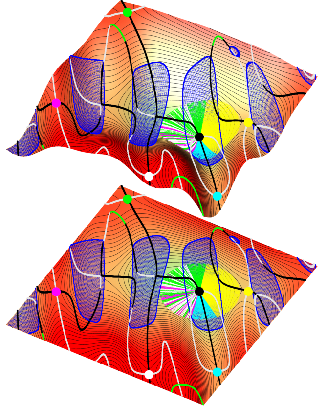
FIG. 9. Same PES and colors as Figs. 1 and 3, but region between x \in [17.1; 20.2] and y \in [25.25; 28.45] . Two CRs need to be crossed to reach the magenta SP from the minimum.
