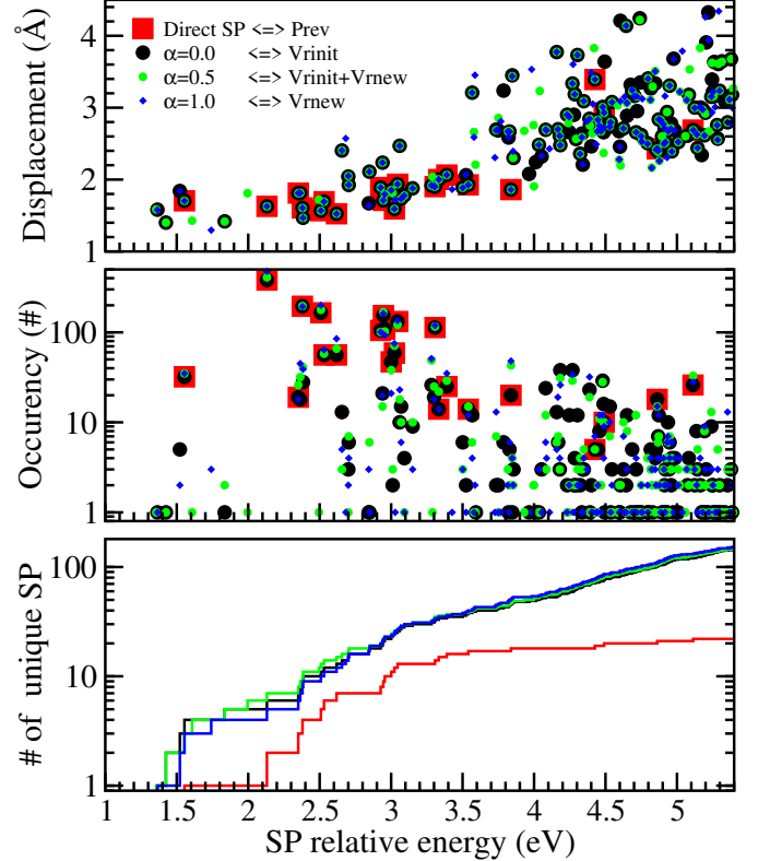
(b) As a function of the SPs energy relatively to the starting minimum: atomic displacement from the initial minimum (top panel), occurrence of each SP (middle panel) and cumulative number of unique saddle points (bottom panel). For clarity, only connected SPs below 5.5 eV and 4.5 Å are plotted, and \mathbf{V}_{min} results are not shown.
