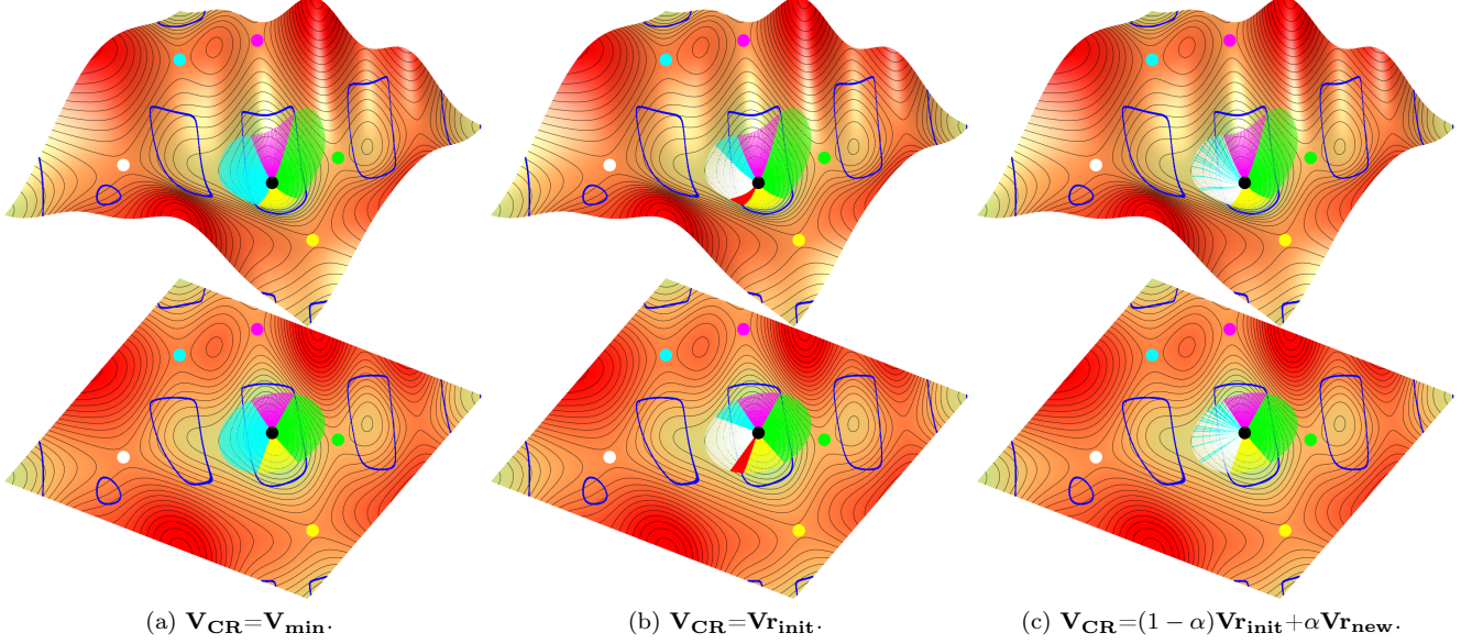
FIG. 3. SPs reached with ARTn starting from the same minimum, as a function of the vector \mathbf{V}_{\text{CR}} used to escape the CRs encountered. Starting from the minimum, 200 searches are launched in uniformly distributed \mathbf{V}_{\text{r}_{\text{init}}} directions, forming a circle in 2D. Each of the 200 slices of the circle around the initial minimum is colored according to the color of the SP reached, with red indicating directions leading to failed explorations (no SP reached due to trajectory cycling in a loop). The \mathbf{V}_{\text{CR}} = \mathbf{V}_{\text{r}_{\text{new}}} case is not shown, as it gives the same kind of results as Fig. 3c, but with a larger number of force evaluations. A video showing the complete exploration leading to these results is given in the Supplementary Material with its gnuplot script.
