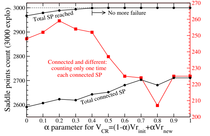
FIG. 8. Count of the number of SP reached using different \mathbf{V}_{\text{CR}} in the convex region.
