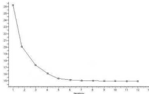
Figure 7: Objective function
