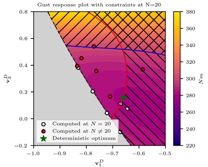
Fig. 6. Isocontours of the gust response showing all used computed simulations projected onto the N = 20 ply space. Constraints are also indicated (black for flutter and red for strain).
