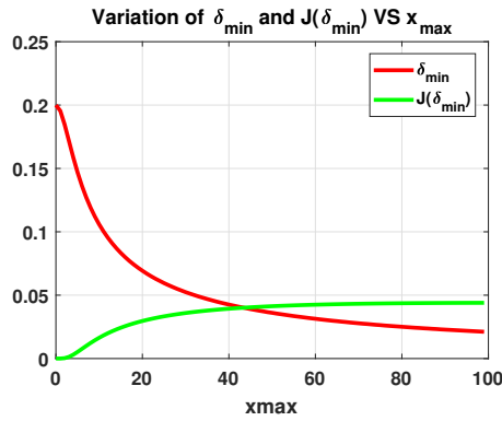
Figure 2: \delta_{\text{min}} and J(\delta_{\text{min}}) for varying x_{\text{max}} .
