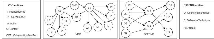
Fig. 3. VDO and D3FEND sub-graphs
