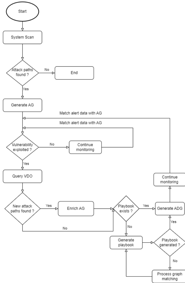
Fig. 2. A flow chart of the ADG generation process
