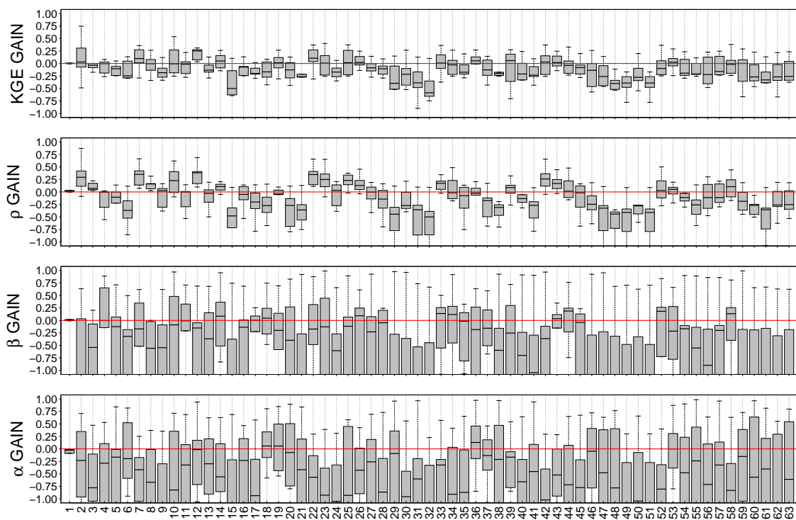
Figure 6. The gain in the KGE and its components computed with the reservoir inflow from the different assimilations. The numbers on the x-axis are the assimilations enumerated in Table A1 and the red lines are the open-loop simulations.
