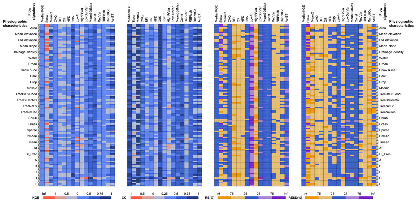
Figure 7. Matrix showing the relation between model capacity to capture flow signatures (colours, where blue is good and yellow/red/purple is poor performance) and physiography of catchments, divided into quartiles (Q1–Q4) for characteristics of the total area upstream of each gauging station with more than 10 years of continuous data (5338 catchments). Descriptions of flow signatures and physiographic characteristics are found in Tables 4–5 and metrics used for model performance in Eqs. (1)–(4).
