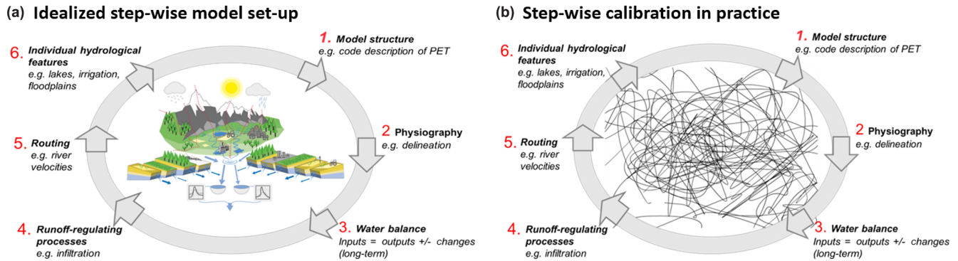
Figure 8. Discrepancy between the idealized procedure for stepwise calibration (a) and the numerous iterations between the steps that appear in reality (b), leading to overall model corrections.
