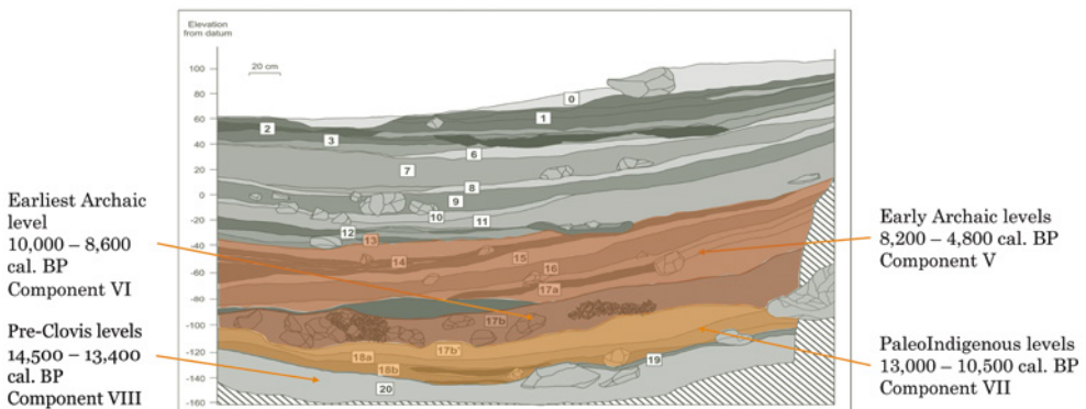
FIGURE 2 West block stratigraphy of Bonneville Estates Rockshelter (after Goebel et al. 2021)
