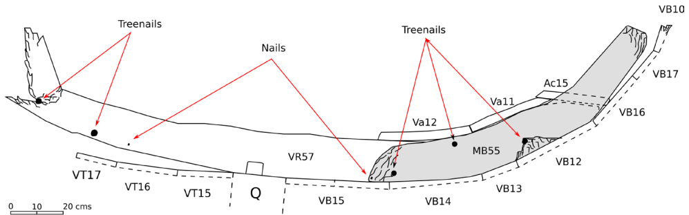
Fig. 1.12. The master frame VR57 (floor timber)/VR55 (futtock) Source: A. Poletto
