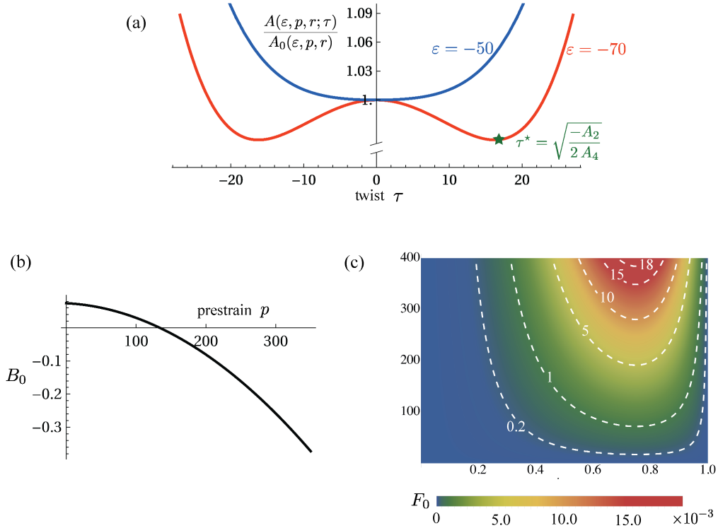
Figure 3.1. Plots of important the energy terms appearing in (2.27–2.29), for Poisson's ratio \nu = 1/2 . (a) Scaled energy per unit length A(p, r, \varepsilon; \tau) / 2 at leading order versus \tau for width ratio r = 2/3 and scaled pre-strain p = -145.58 : the profile is convex for moderate end-to-end shortening (scaled axial strain \varepsilon = -50 , blue curve) and becomes non-convex for more severe end-to-end shortening ( \varepsilon = -70 , red curve); the loss of convexity (onset of twist buckling) takes place at \varepsilon = -55.1348 . (b) Incremental gradient modulus B_0 = B(p, r = 2/3; \tau = 0) evaluated in the planar configuration ( \tau = 0 ) as a function of pre-strain p . Later in this paper, we will connect the change of sign in B_0 to the transition from long- to short-wavelength buckling. (c) Fourth-order term F_0(p, r) > 0 is always positive. This warrants that the overall energy remains positive against very short-wavelength perturbations ( q \rightarrow \infty ), even when the second-order gradient modulus B_0 is negative.
