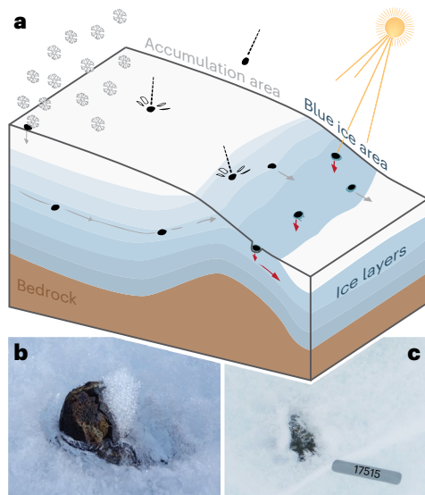
Fig. 1 | Antarctic meteorites in blue ice areas. a , Schematic representation of the meteorite concentration mechanism, with a supply of meteorites through ice flow and direct infall and loss of meteorites through melting from the surface into the ice (sinking, red arrows). The sinking of meteorites is caused by (increased) warming of the dark meteorites (especially those with high metal contents and thermal conductivity) under solar radiation, causing the underlying ice to melt, and hence the meteorite to sink into the ice. b , The Hutchison Icefield 18033 meteorite (49 g) collected as part of the Lost Meteorites of Antarctica Project 10,24 . c , Meteorite MIL 07710 (147 g) fully enclosed in ice, collected as part of the Antarctic Search for Meteorites (ANSMET) programme (the number in the photo is used for documentation in the field). A column of clear, bubble-free ice above the meteorite was observed during the field mission (transparent on photograph), indicating that the meteorite sunk through melting underlying ice that refroze as superimposed ice above the sample 16 . Credit: b , Katherine Joy, Lost Meteorites of Antarctica Project 10,24 ; c , Ralph Harvey, ANSMET programme.
