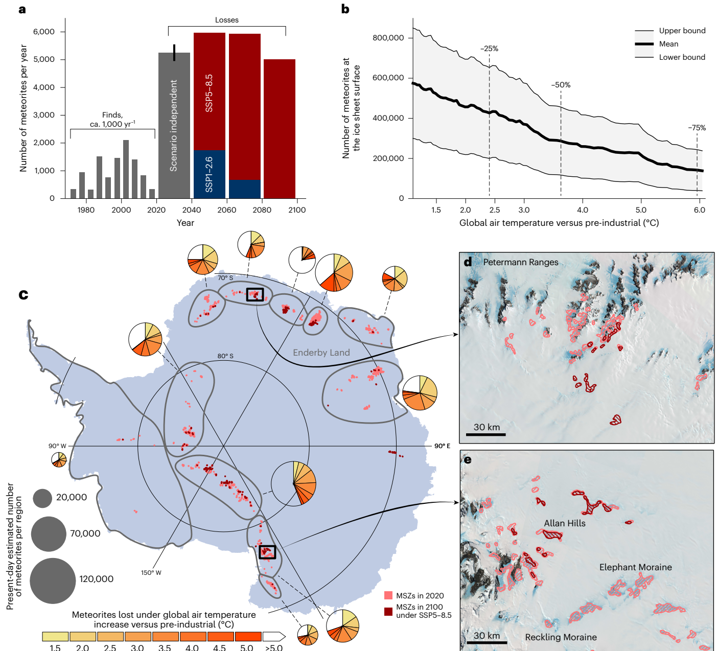
Fig. 2 | Projected evolution of meteorites in Antarctica under climate warming. a , Antarctic meteorite finds up to 2020 (that is, including January or February 2019, not including 2020) documented in the Meteoritical Bulletin 17 (averaged over 5 yr intervals) and predicted future loss rates (averaged over 20 yr intervals) for a low-emissions scenario (Shared Socio-economic Pathway (SSP)1-2.6) and a high-emissions scenario (SSP5-8.5) (Supplementary Fig. 1). Estimates for the two emissions scenarios start to deviate from 2052; therefore loss rates for 2020–2040 are averaged for the two scenarios with the error bar representing the lower and upper estimates. b , The projected number of meteorites remaining at the ice sheet surface in relation to global air temperature increase with respect to pre-industrial levels (1850–1900; Supplementary Fig. 3). The graph displays the average estimate (bold line) and both the lower and upper bounds (grey shading; Methods), and indicates under which temperature increase 25%, 50% and 75% of the meteorites are lost. c , Continent-wide estimate of meteorite stranding zones (MSZs) in 2020 and in 2100 under SSP5-8.5 (both exaggerated
