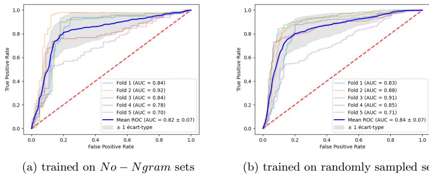
Fig. 3: ROC of 5-folds agnostic classifiers
