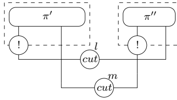
Fig. 7. Counter-example of confluence of cut reduction on proof structures.
