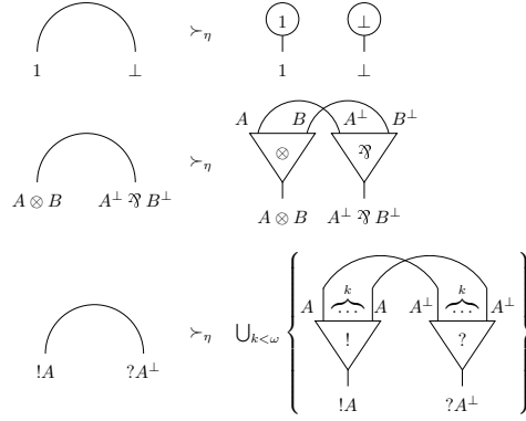
Fig. 3. Cut-elimination rules ( \beta -reduction).
