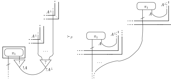
Fig. 6. Cut-elimination rule for promotion.
