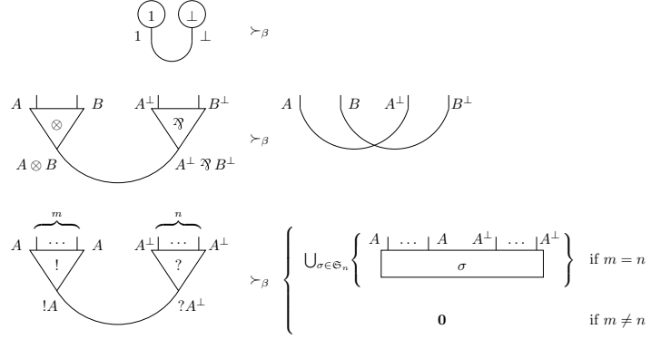
Fig. 3. Cut-elimination rules ( \beta -reduction).
