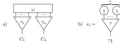
Fig. 5. a) Decomposition of a normal simple net. b) Definition of the net \epsilon_i , i \in \mathbb{N} .
