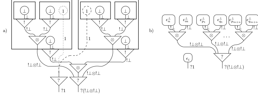
Fig. 7. a) Example 1 of non-separable proof-nets: \pi_1 is defined by considering the dotted wire and cell, instead \pi_2 by considering the dashed ones. b) Definition of \alpha \langle i, n, m, p_1, q_1, \dots, p_{n+m}, q_{n+m} \rangle , where \epsilon_i is the simple net of Fig. 5b.
