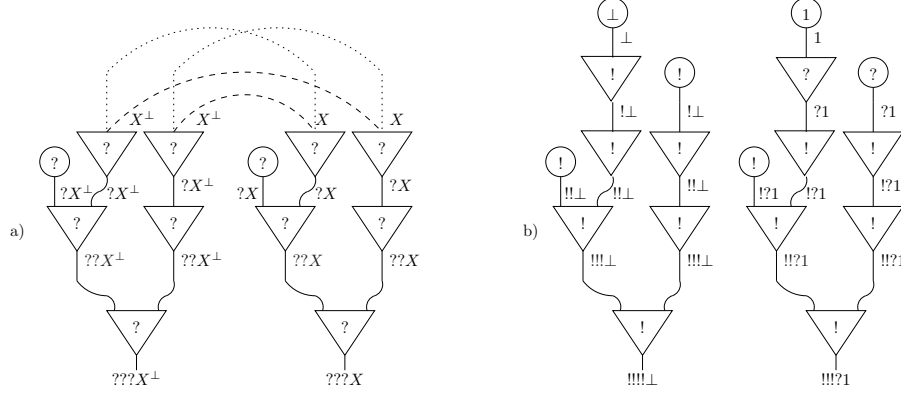
Fig. 8. a) Example 2 of non-separable proof-nets: \pi_1 is defined by considering the dashed wires, instead \pi_2 by considering the dotted ones. b) Simple net separating \pi_1^* , \pi_2^* of a)
