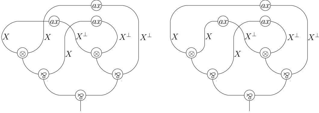
Fig. 6. Example of proof nets \pi_1, \pi_2 with conclusion ((X \otimes X) \wp X) \wp (X^\perp \otimes X^\perp) \wp X^\perp .
