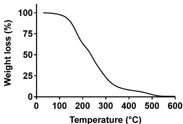
Figure 3. Thermogravimetric curve from Chinese star anise whole seedpod oil (CSAO) under the heating rate of 10 °C/min and 10 mL/min oxygen flow.
