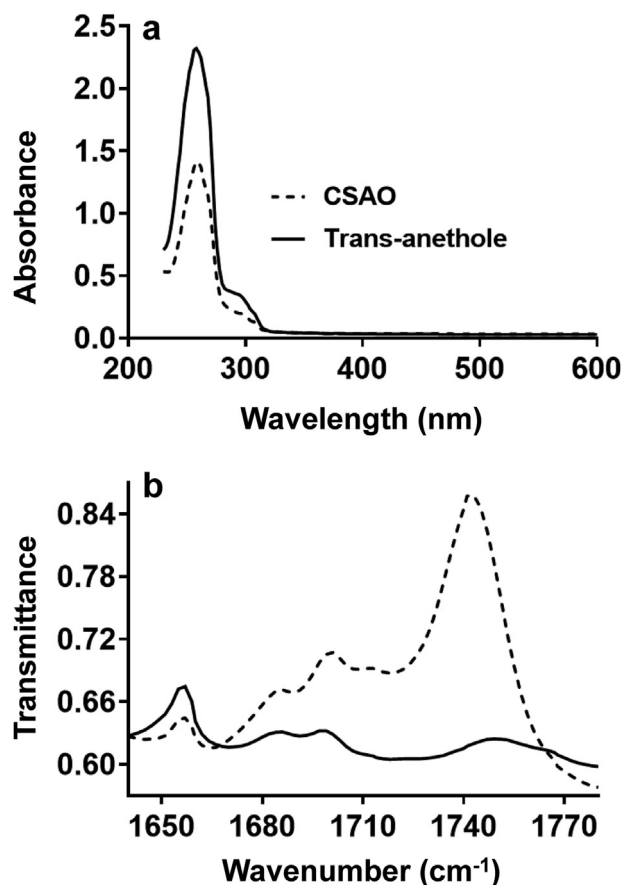
Figure 2. (A) UV-vis absorption spectra of Chinese star anise whole seedpod oil (CSAO) and standard trans-anethole, obtained at 230–700 nm. (B) Expanded FTIR spectral region that exhibits the observed differences between CSAO and standard trans-anethole.
