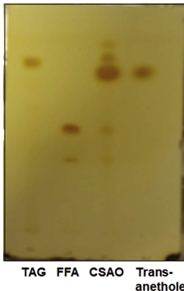
Figure 1. TLC analysis of unconventional Chinese star anise whole seedpod oil (CSAO) neutral lipids as revealed by staining with iodine. TAG, FFA and trans-anethole were included as standards.
