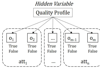
Figure 2: Naive Bayes model for diagnosis. The value of quality profile has influence over the different attributes' observations. Knowing the quality profile value guarantees independence between observations. Observations o_k ( k \in [1, m] ) are booleans representing whether or not an attribute takes a value.
