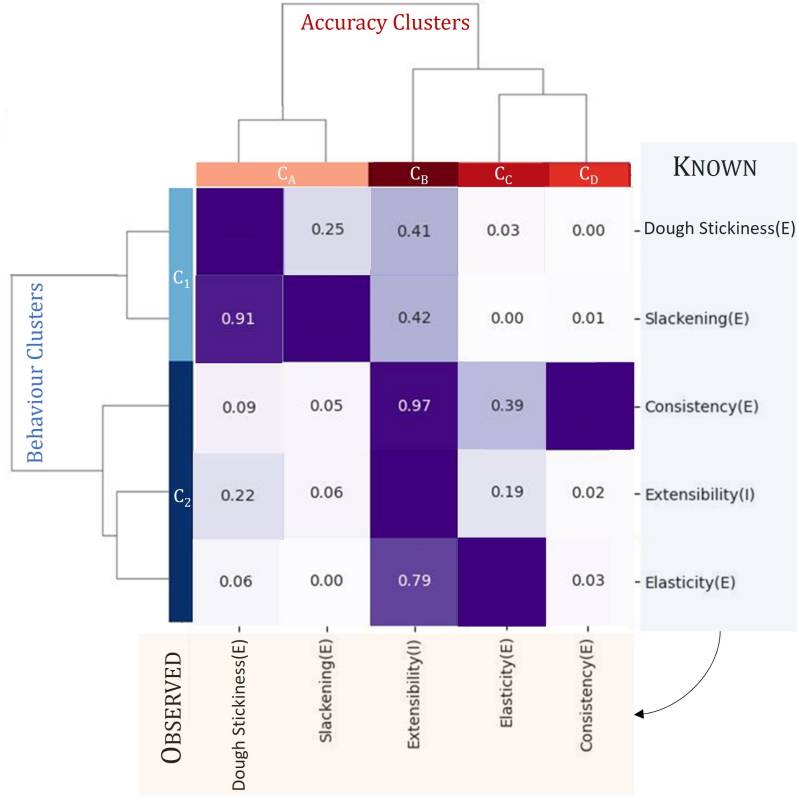
Figure 3: Clustermap of probabilities for the reduced example. Each case (i; j) (row i , column j ) indicates the probability P(j|i) , i.e. the probability of the OBSERVED defect j when defect i is KNOWN. Probabilities between two identical observations are not indicated, since their value is 1 by definition. Behaviour clusters define C_1 and C_2 . Accuracy clusters define C_A , C_B , C_C and C_D .
