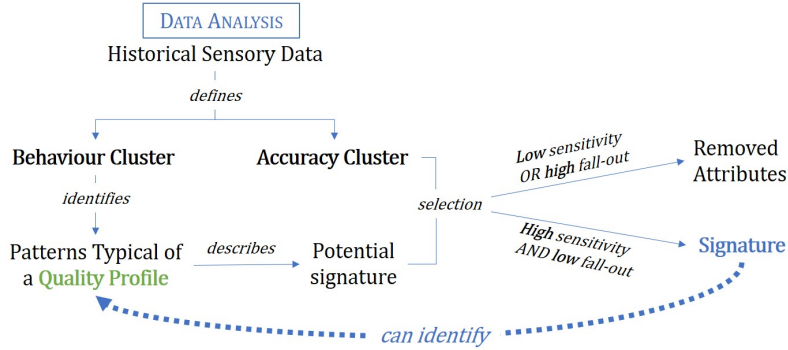
Figure 4: Overview of the historical sensory data analysis that allows signatures to be linked to quality profiles. Behaviour clusters are used to identify patterns describing potential signatures; accuracy clusters trim the potential signatures to keep only observations with high sensitivity and low fallout for their assigned quality profile.
