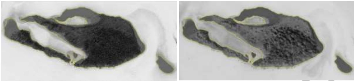
FIGURE 2. NDWI (left), DDWI (right) and extracted shoreline (yellow) of Tahuna iti (2016 Pléiades)
