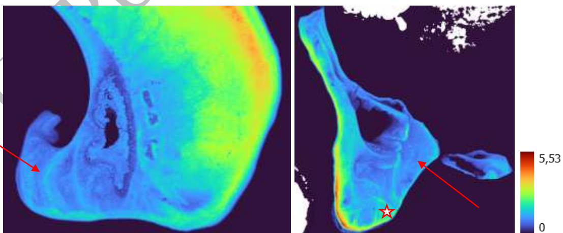
FIGURE 15. 2017 lidar DTM of Horoāterā (left) and Rimatu'u-Tahuna iti (right)
