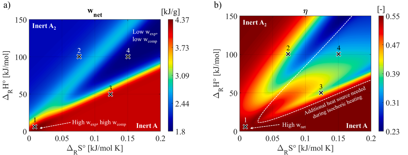
Fig. 9. Overall performance of the Stirling cycle operating with theoretical ideal gas mixture A_{2(g)} \rightleftharpoons 2A_{(g)} for different reaction coordinates (\Delta_R S^o, \Delta_R H^o) . (a) Net specific work output, w_{net} . (b) Thermal efficiency, \eta . Four chemically reactive fluids are marked for further T-q diagram analysis.
