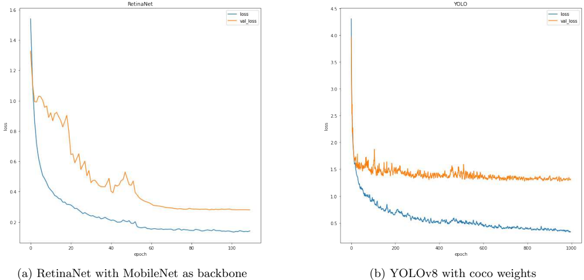
Figure 6: Graphs of loss function. The x-axis represents the number of epochs during the training process. The y-axis represents the value of the loss function. The goal during training is to minimize this value, as a lower loss indicates better alignment between the model's predictions and the actual data.
