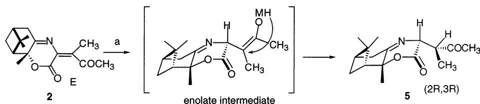
Scheme 3. Reagents and conditions: (a) Pd(OH) 2 /C, EtOH, rt, 5 , 64%.
