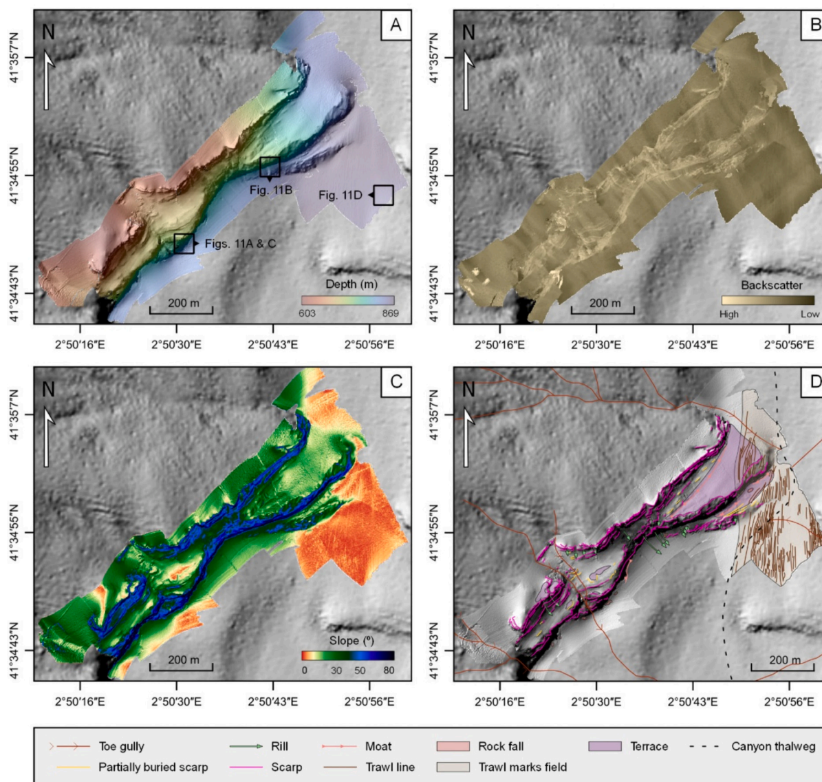
Fig. 10. Western flank area mapped at 80 cm resolution using the H-ROV Ariane . (A) Shaded relief map showing the location of the images acquired with the ROV Liropus in this region. (B) Backscatter map. Light colors represent higher intensity values matching with the vertical rockwalls. (C) Slope map measured in degrees. The blue colors show slope values of >50^\circ coinciding with vertical walls. (D) Geomorphological map that shows the morphologic features visible only at this very fine-scale inferred from the previous three maps. Refer to supplementary material (Fig. S2) for a three-dimensional perspective of the maps.
