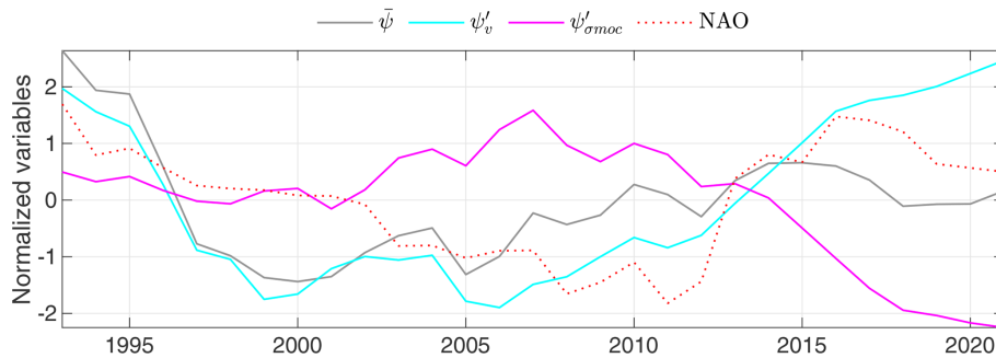
Figure 11. Winter NAO (dotted red line), \bar{\psi} (grey), \psi'_v (cyan) and \psi'_{\sigma_{moc}} (magenta). \bar{\psi} , \psi'_v and \psi'_{\sigma_{moc}} are the average of CORA, EN4 and GloSea5. Time series were normalized by their standard deviations and low-pass filtered using a moving mean with a 60-month window.
