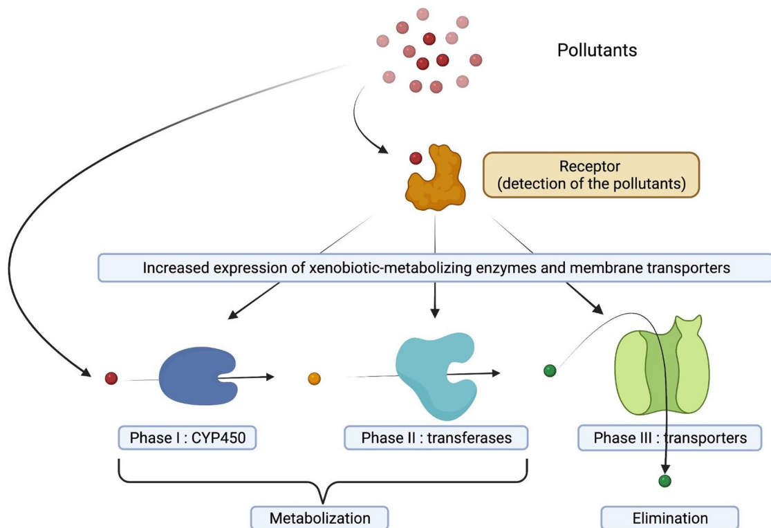
Figure 1. A general presentation of xenobiotic metabolism. Three phases are considered as essential, the first 2 steps corresponding to the activation and conjugation of xenobiotics leading to the production of metabolites, which are generally more hydrophilic. Therefore, a necessary third step involving membrane transporters leads to the elimination of the metabolites from the cell and subsequently, from the body (urines, sweat. . .).
