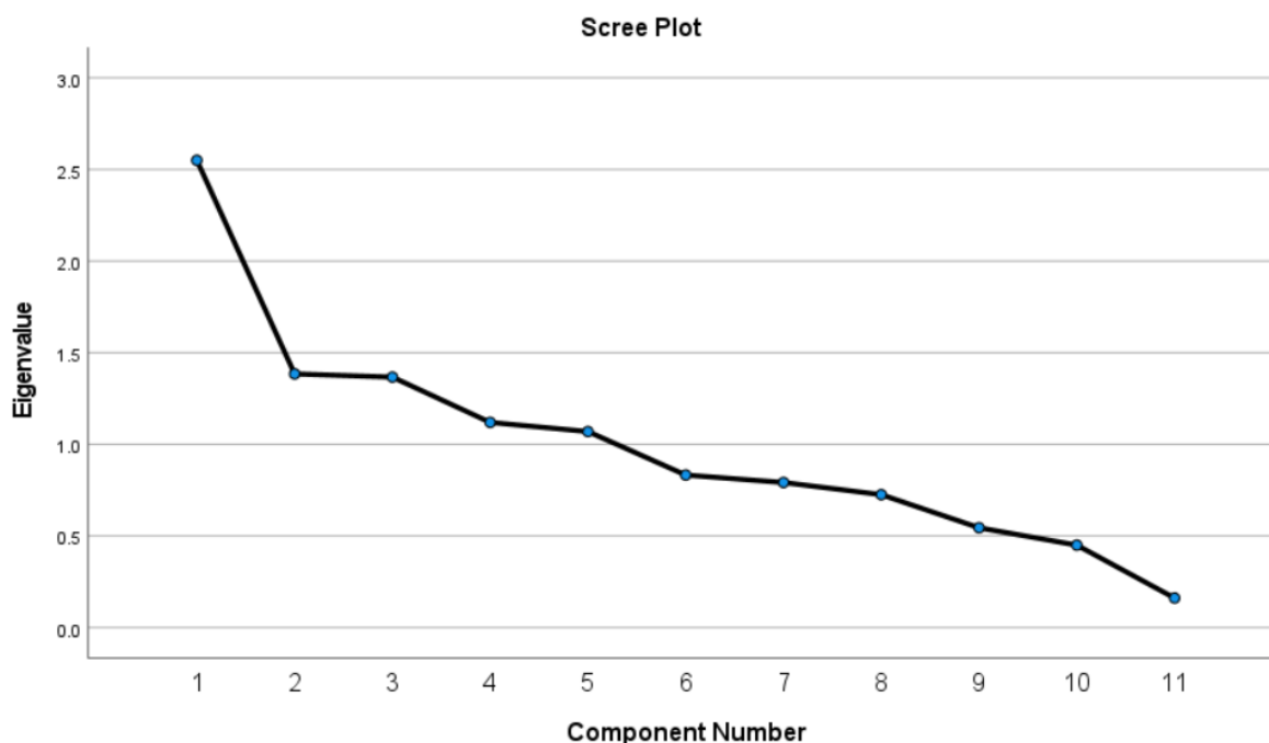
Fig. 1. Scree plot
