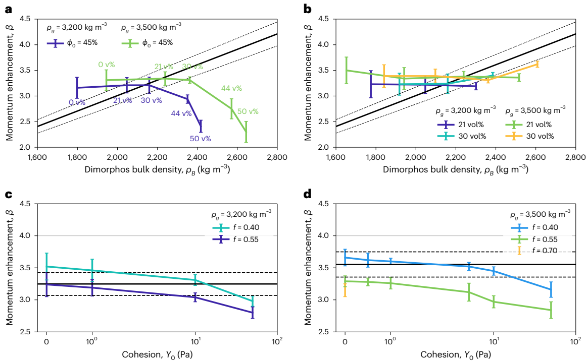
Fig. 1 | Momentum enhancement \beta as derived from SPH simulations. a–d , Continuous black lines show the \beta dependence on Dimorphos’s bulk density \rho_B derived from dynamical simulations 7 ( 1\sigma uncertainty is shown by the dashed lines). Data points that cross a solid black line are consistent with the measured \beta from the DART impact. The uncertainty for each simulated data point (vertical bars) was calculated from the absolute difference in \beta calculated from two different methods (‘Momentum-enhancement calculations’ in Methods). a , \beta as a function of \rho_B for cohesionless targets with the same dimensions as Dimorphos 1 and with boulder volume fractions ranging from 0 vol% (no boulders larger than 2.5 m) to 50 vol%. For fixed target volume (0.00181 km 3 ) and fixed matrix porosity ( \phi_0 = 45\% ), the mass and bulk density of Dimorphos vary with the boulder packing. b , \beta as a function of \rho_B for cohesionless targets with the
