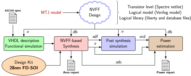
Fig. 3. ASIC design flow implemented to design the ASCON non-volatile circuit
