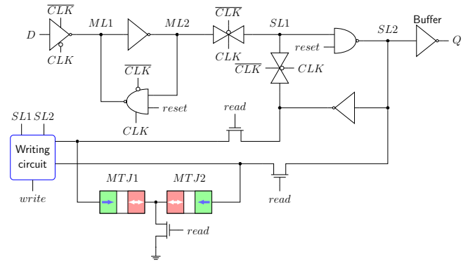
Fig. 4. Non-volatile flip-flop schematic
