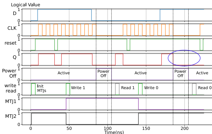
(b) NVFF logical simulation performed with Questasim
