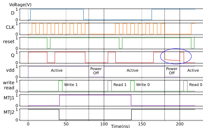
Fig. 5. (a) NVFF electrical simulation issued from Spectre
