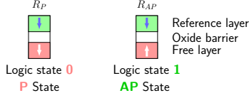
Fig. 2. MTJ with P and AP states
