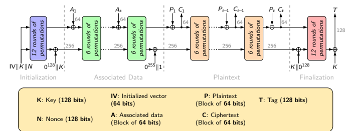
Fig. 1. Encryption part of ASCON-128
