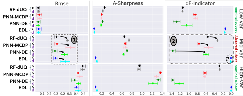
Fig. 2: Subset performances for one experimental setup on real data. Control and degraded models are denoted by c and d .
