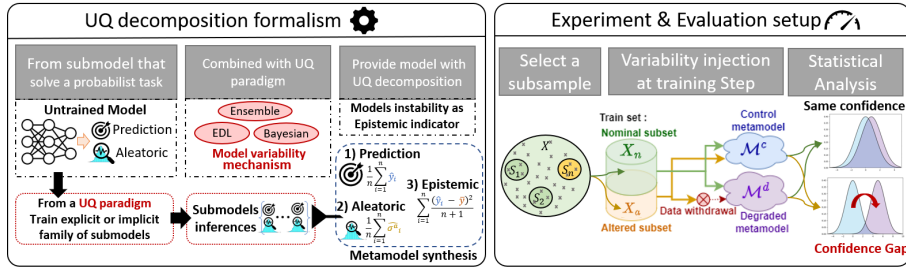
Fig. 1: Disentangled UQ framework and the experimental setup
