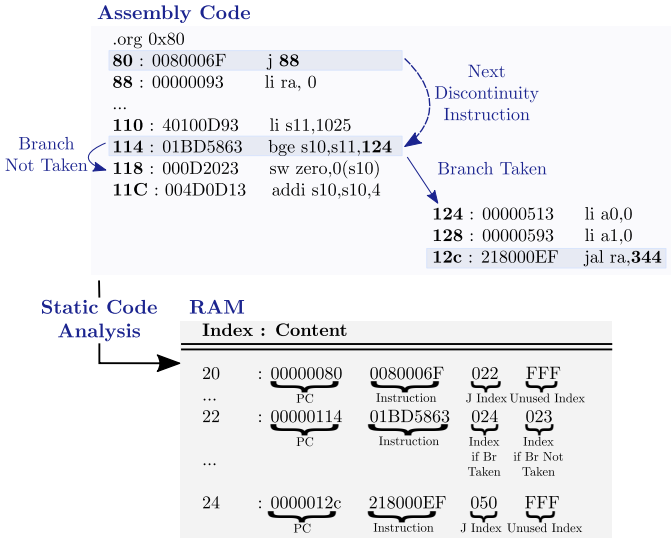
Fig. 2: Metadata content stored in RAM.
