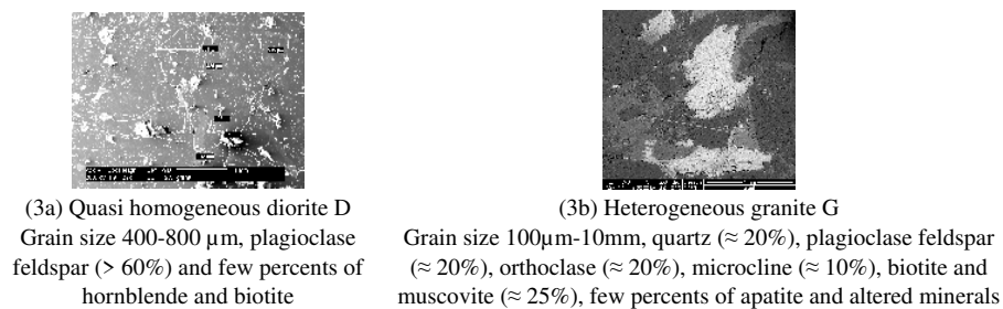
Figure 3. SEM (Scanning Electron Microscopy) images of the two specimens
