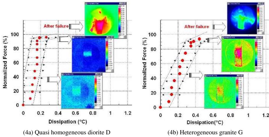
Figure 4. Different stages of heat dissipation describing the process of the damage extent in the specimen. Graphical determination of the threshold of acceptable damage TAD of tested materials subject to unconfined loading up to failure.
