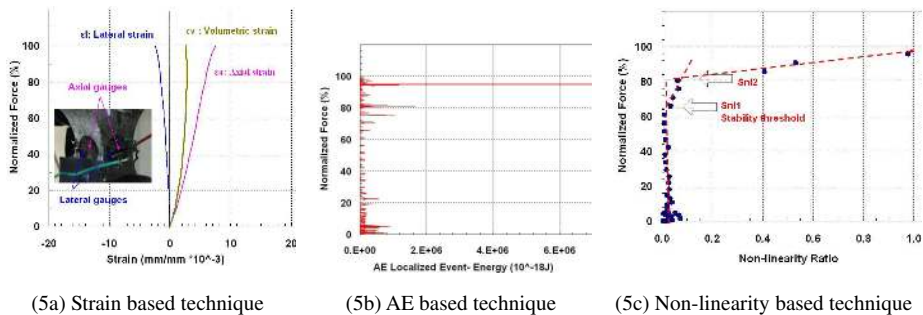
Figure 5. Experimental results obtained when using other testing techniques on brittle rock specimen.
