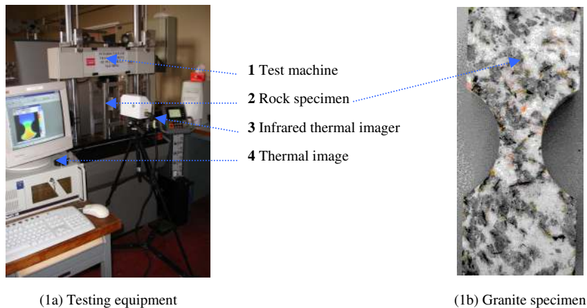
Figure 1. Experimental setup of infrared thermovision on rock specimen
