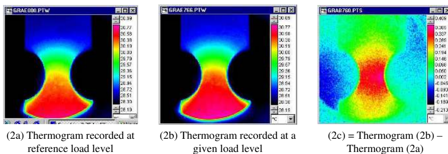
Figure 2. The differential infrared thermography enhances the localization of intrinsic dissipation (temperature changes are given in °C)
