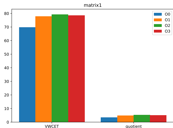
Fig. 8: matrix1 VWCET and quotient
