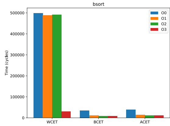
Fig. 1: bubble sort execution times
