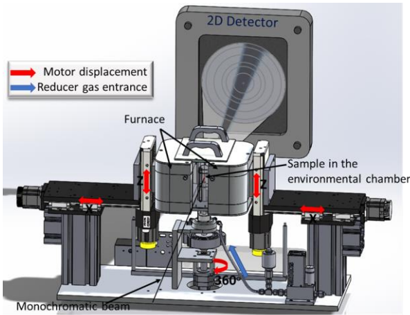
Figure 3. Experimental setup used at DESY at beamline P21.02.
