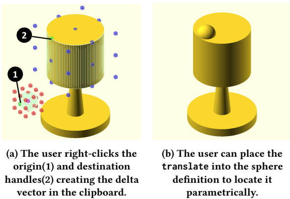
Figure 4: Delta vector allows users to place one object’s handle relative to another object’s handle.
