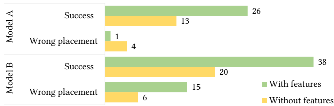
Figure 10: Outcomes of attempts to verify translate using the modified version of OpenSCAD
