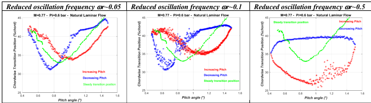
Figure 30: Effect of the pitch oscillation frequency on the transition behaviour : M=0.77 ;pitch = 1^\circ \pm 0.5^\circ . The green line represents the steady transition variation from quasi-steady polars.
