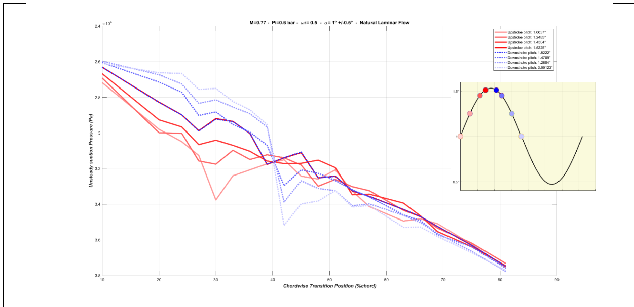
Figure 31: Snapshot at different times of the upper section unsteady pressure distribution during a pitch oscillation in free transition flow. (reddish curves = upstroke times; blueish curves =downstroke times). M=0.77 ; \bar{\omega}=0.5 ;pitch = 1^\circ \pm 0.5^\circ
