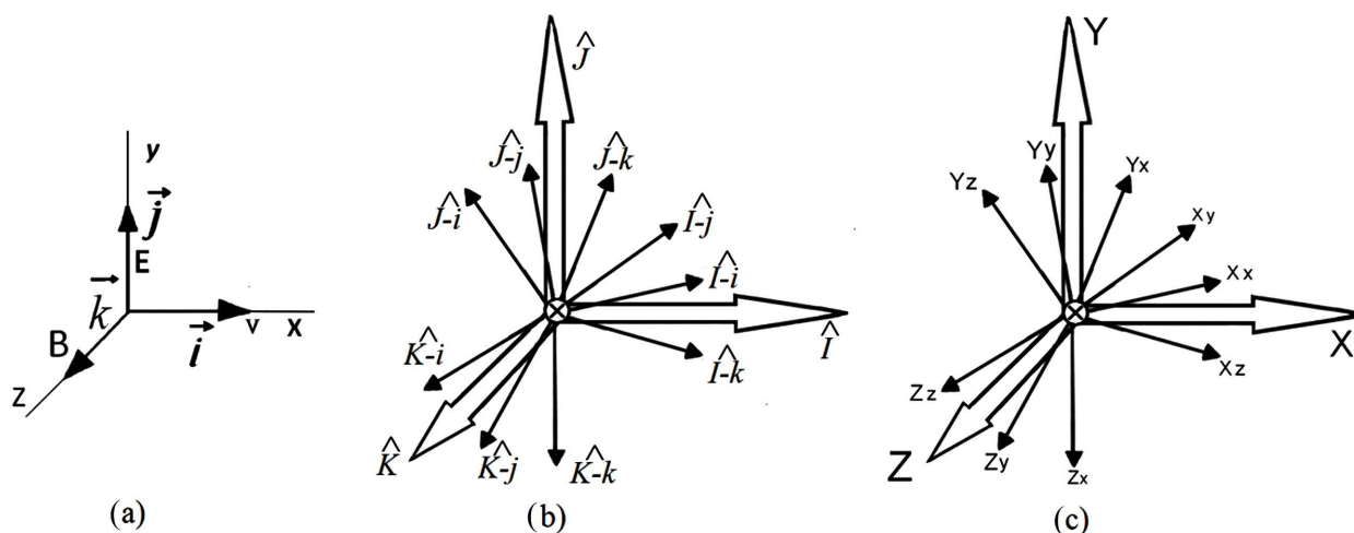
Figure 1. The Major and minor vector sets applicable to the trispacial geometry.
