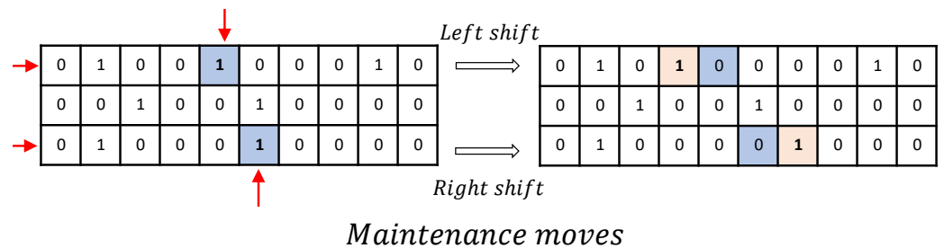
Figure 5. Illustrative examples of right and left shift moves.
