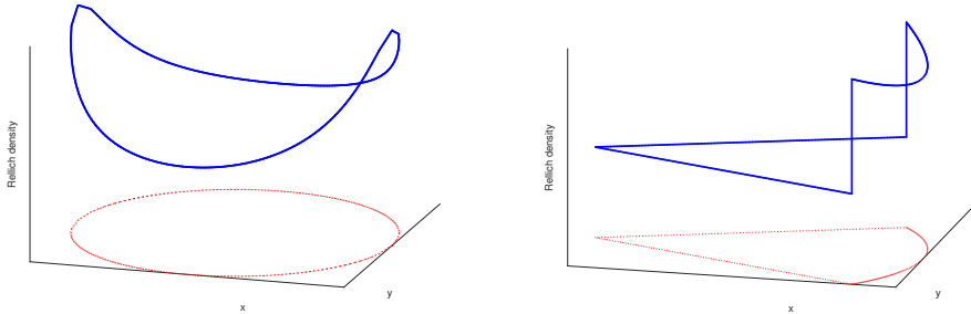
Figure 1: Plot of two Rellich densities (continuous line): for an ellipse (dotted line, left) and for an angular sector (dotted line, right).
