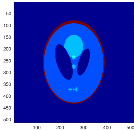
Figure 5: Initial source p_0 .
