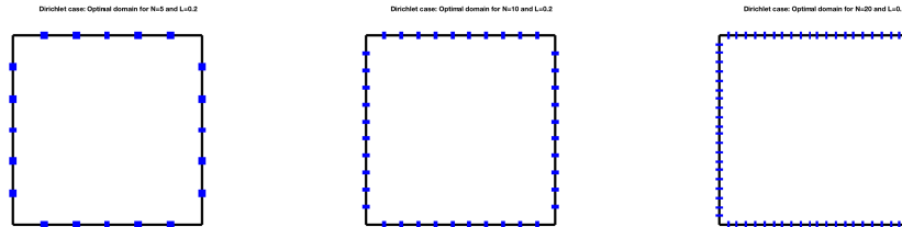
Figure 2: \Omega = [-\pi/2, \pi/2]^2 and L = 0.2 . Examples of maximizers a_N^* for J_N and (from left to right) N \in \{5, 10, 20\} . The bold line corresponds to the set \Gamma = \{a_N^* = 1\} .
