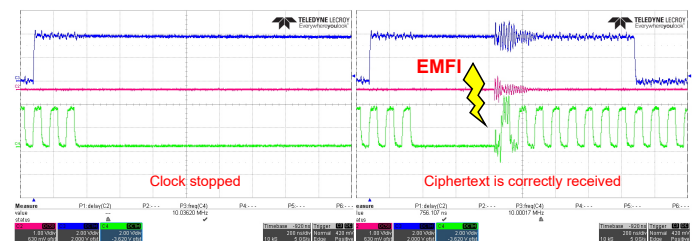
Fig. 2: Freezing the AES clock signal.
