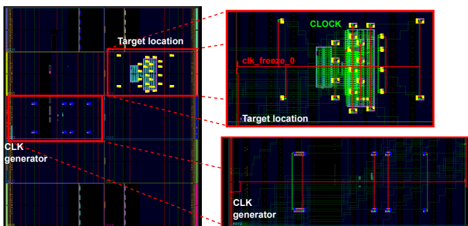
Fig. 6: Target’s floorplan from Vivado showing the sensor’s distribution within the design logic blocks.
