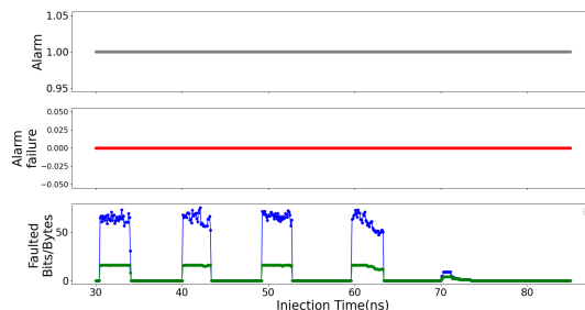
Fig. 10: EMFI results at 200 MHz (+300 V voltage pulse).
