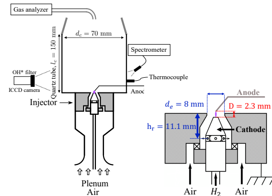
Fig. 1: Left : Schematic view of the SICCA-H2 experimental setup. Right: Schematic view of the CFI-X3 cross-flow injector, equipped with a 1-mm diameter tungsten electrode for NRP discharges.
