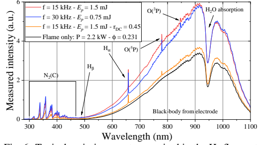
Fig. 6: Typical emission spectra acquired in the H_2 flame at P_{th} = 2.2 kW and \phi = 0.231 . Spectra are acquired during 50 ms and averaged 40 times. The black line is acquired without the plasma. The red and orange lines are acquired with the 15 kHz – 1.5 mJ plasma, applied respectively continuously and with a duty-cycle ratio of 0.45. The blue line is acquired with the 30 kHz - 0.75 mJ plasma applied continuously.
