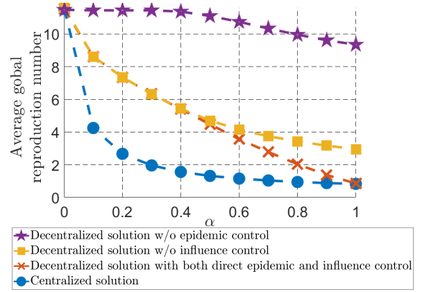
(a) Plot of \sum_{n=0}^N \frac{\rho \left( \mathbf{D}_\gamma^{-1} \left( \mathbf{B}^0 - \mathbf{U} + \text{Diag}(\theta(n)) \hat{\mathbf{B}} \right) \right)}{N+1} vs \alpha .
