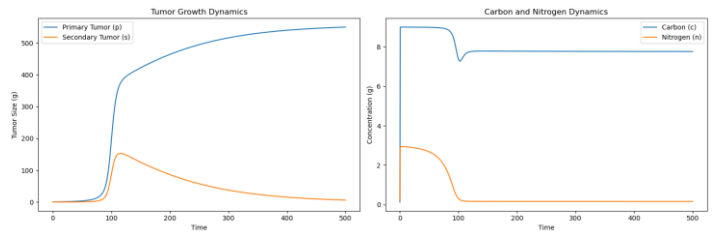
Figure 3 – Breast tumour competition occurs within C:N ratio similar to figure 2. This competition is characterized by the interplay of (a) tumour growth dynamics, (b) carbon dynamics, and nitrogen dynamics. The dynamics are further delineated as follows \beta_1 = 0.0693 , \beta_2 = 0.077 , \alpha_1 = 0.4 , \alpha_2 = 0.5 .
