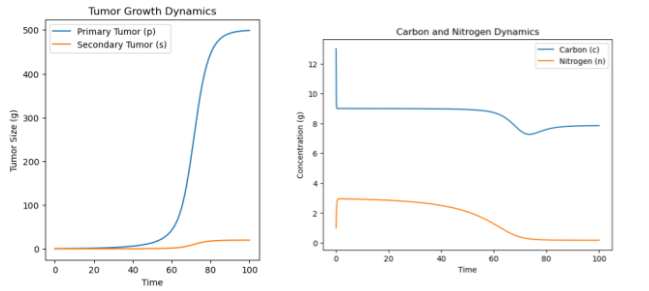
Figure 1 - Tumour competition occurs within a framework of homeostatic C:N ratios at 3:1 (equivalent to 9.0 for carbon and 3.0 for nitrogen). This competition is characterized by the interplay of (a) tumour growth dynamics, (b) carbon dynamics, and nitrogen dynamics. The dynamics are further delineated as follows ( \beta_1 = \beta_2 = 0.077 , \gamma_1 = \gamma_2 = 0.20 , \omega_1 = \omega_2 = 1 ).
