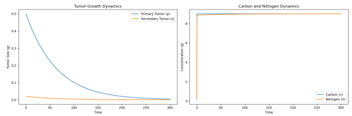
Figure 4 – Breast tumour competition occurs C:N ratio similar to figure 2. This competition is characterized by the interplay of (a) tumour growth dynamics, (b) carbon dynamics, and nitrogen dynamics. The dynamics are the same as figure 2, except C_B = N_k = 9
