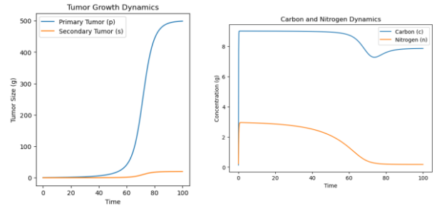
Figure 2 – Breast tumour competition occurs within C:N percentages of 25.7% and 41.6% of total biomass, respectively. This competition is characterized by the interplay of (a) tumour growth dynamics, (b) carbon dynamics, and nitrogen dynamics. The dynamics are the same as figure 1.
